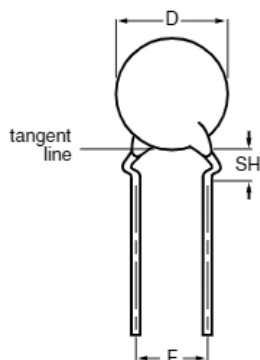
Capacitors with outside kink lead spacing
