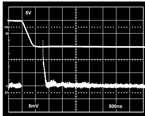
Figure 36. Settling Characteristics 0 V to -10 V Step Upper Trace: Output of AD712 Under Test (5 V/Div) Lower Trace: Amplified Error Voltage (0.01%/Div)
