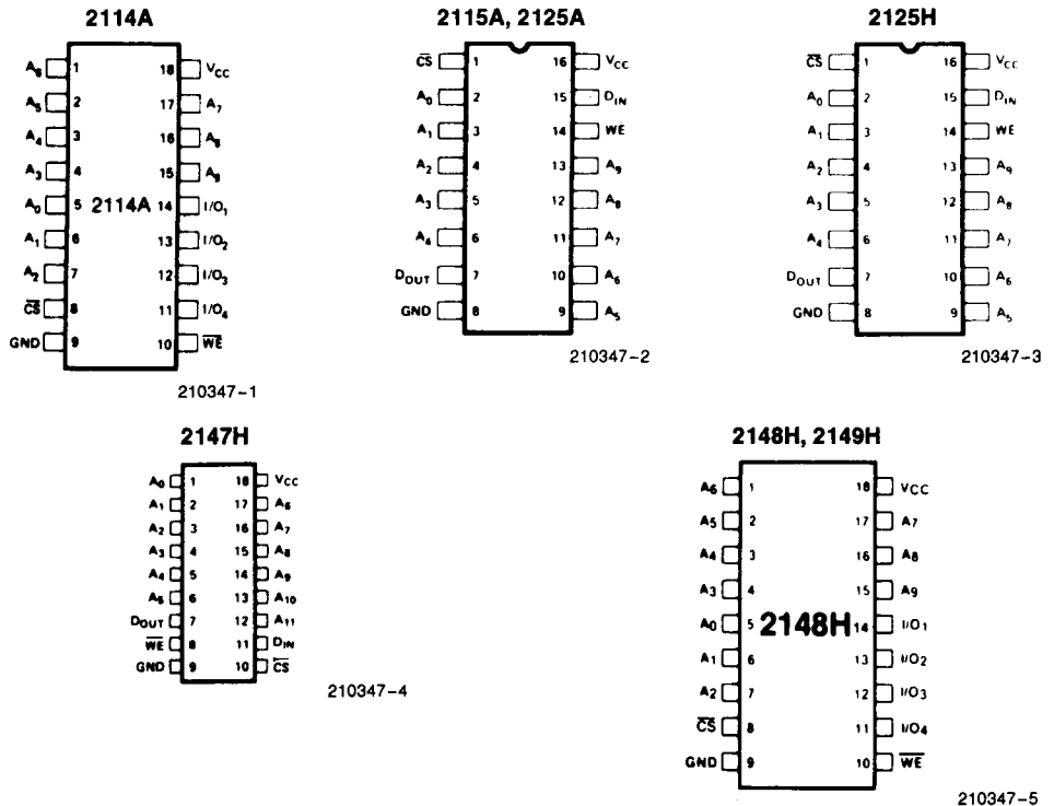
Pin Configuration
