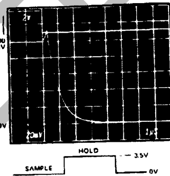
ACQUISITION TIME +100mV to 0V
