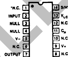
14-PIN DIP (Y-Suffix) 14-PIN EPOXY DIP (P-Suffix)
